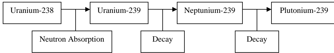
Fig. 2 - Uranium-238 changing to Plutonium 239
