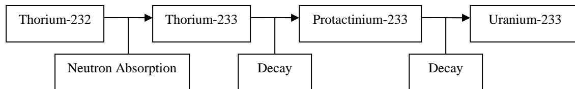
Fig. 1 - Thorium-232 changing into Uranium-233
