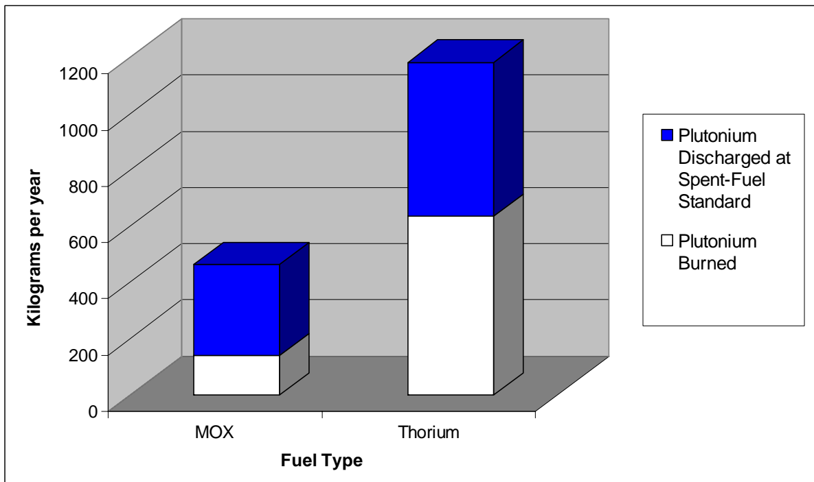
Fig. 7 – Thorium fuel vs. MOX fuel
