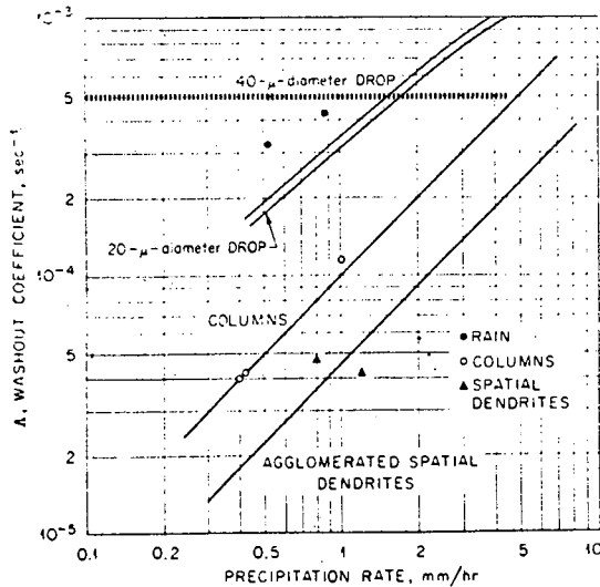
Fig. 7 Washout coefficients for inorganic iodine in process-plant stack gases in rain and snow. (From Ref. 37.)
