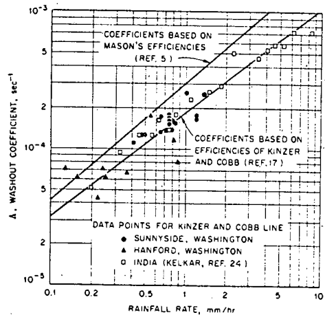
Fig. 5 Washout coefficients for a^2\rho = 42 only, calculated from spectra measured in Washington and India based on theoretical efficiencies from Mason 3 and measured efficiencies of Kinzer and Cobb. 17
