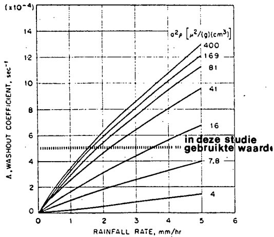
Fig. 4 Washout coefficients for unit density particles vs. rainfall rate and a^2\rho [ \mu^2/(g)(cm^3) ], where a and \rho are the radius and density of the particles. These calculations are based on Best's 22 spectra and Langmuir's 11 target efficiencies. (Adapted from Ref. 6.)
