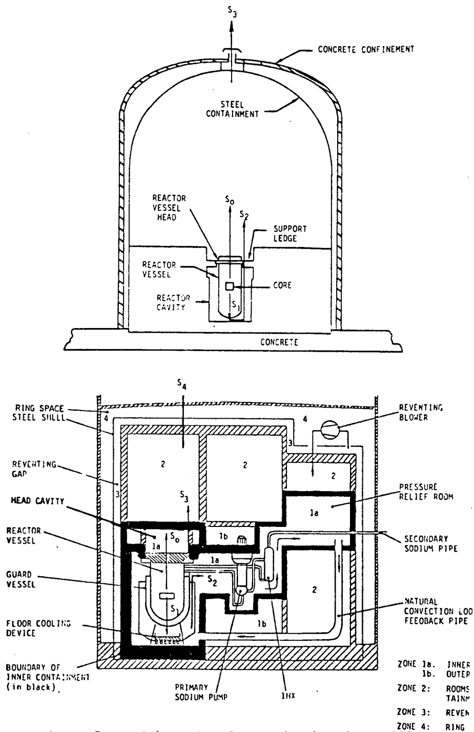
Figuur 5.1 Schematic of CRBR (top) and SNR-300 (bottom) Containment System and the Radionuclide Source Terms S_0 , S_1 , S_2 , S_3 and S_4 in the Post-HCDA Phase.
