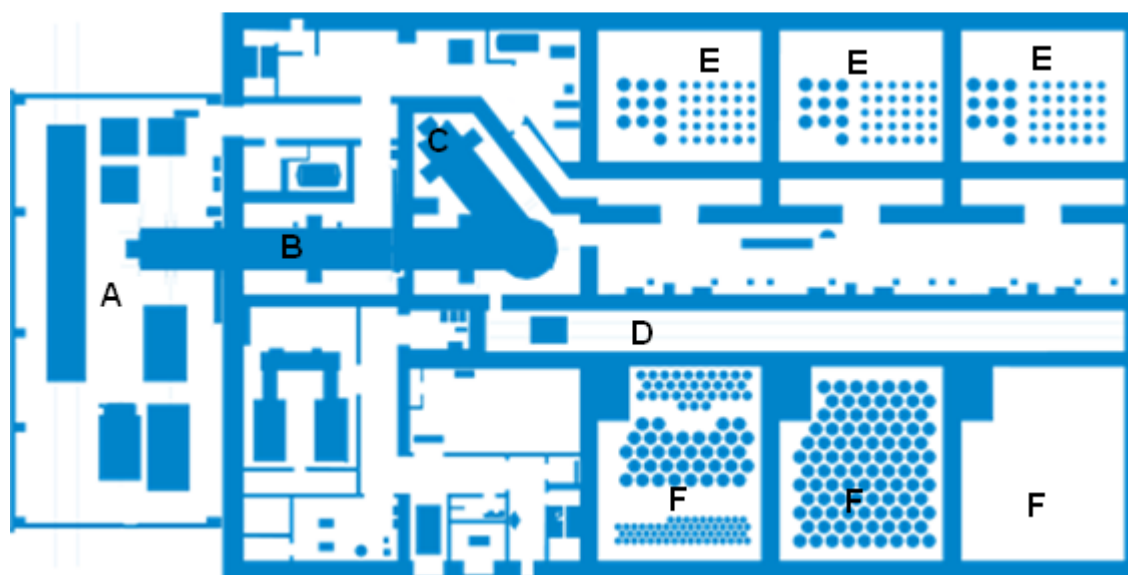
Figure 1.4 HABOG floor plan
