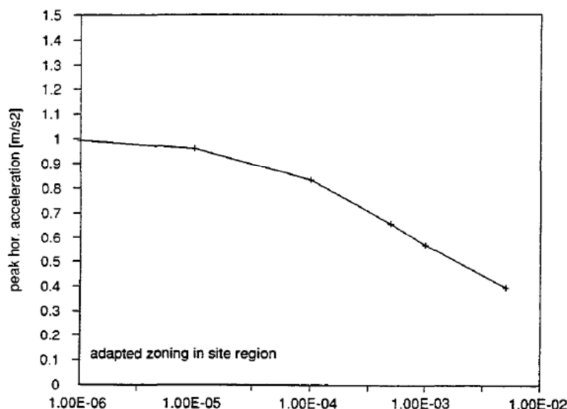
Figure 2.3 Probability of exceedance per year (X-axis) vs. horizontal peak acceleration (Y-axis)
