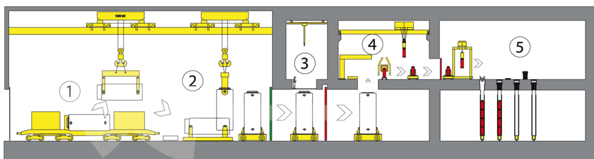
Figure 1.9 Processing of V-HPW . Step 1: inspection of transport container; Step 2: positioning of transport container; Step 3: unbolting of cover (cover not removed) and sampling for contamination; Step 4: unloading of transport container and inspection of canisters; Step 5: storage in cylinder (well)
