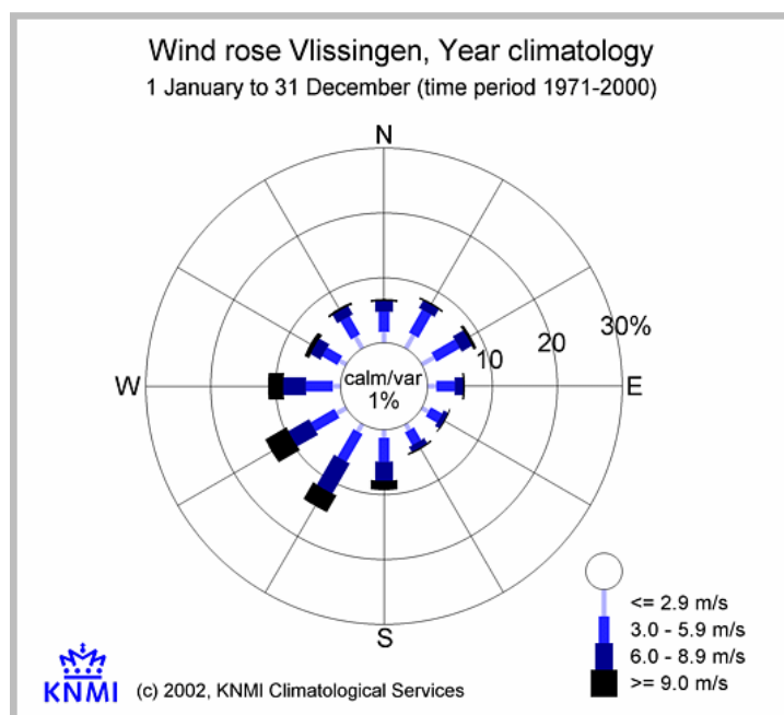
Figure 6.3 Wind rose, measured at KNMI station Vlissingen
