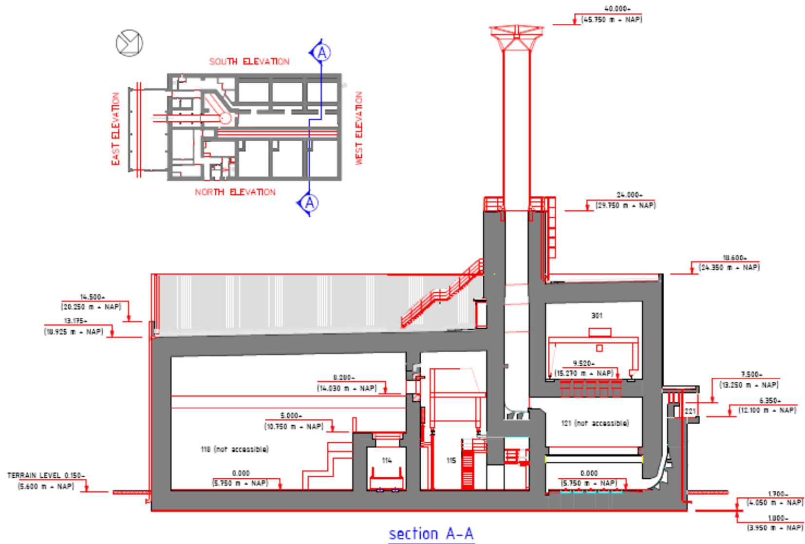
Figure 3.3 Level indications of the HABOG building (cross section). Room 118 contains the non-HPW, room 121 the HPW.
