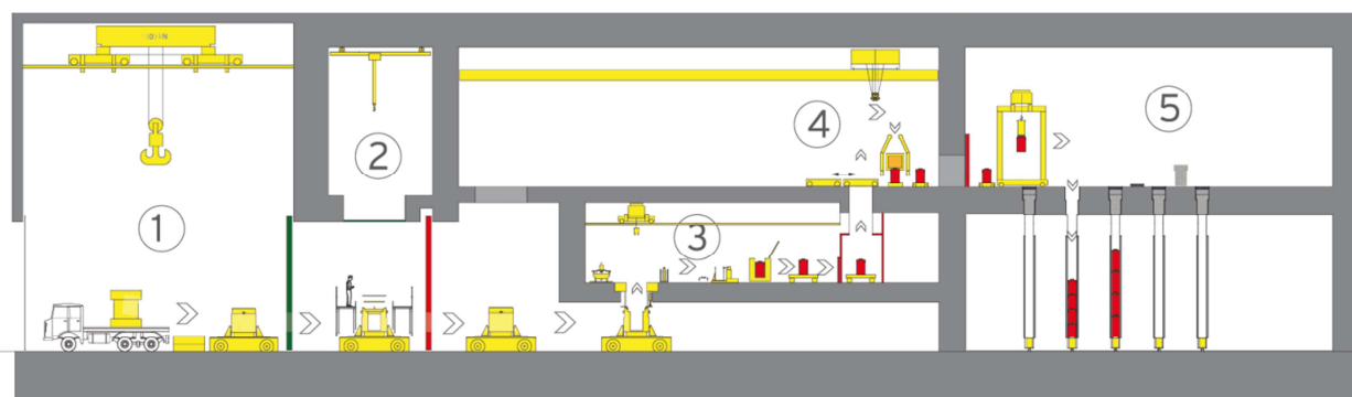
Figure 1.8 Processing of RR-HPW . Step 1: inspection of transport container and removal of shock absorbers; Step 2: unbolting of cover (lid not removed) and sampling for contamination; Step 3: RR-fuel is repacked in storage canisters, canisters are cleaned; Step 4: inspection of canisters; Step 5: storage in cylinder (well)
