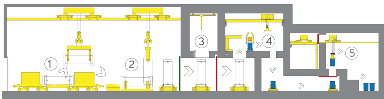
Figure 1.10 Processing of non-HPW . Step 1: inspection of transport container; Step 2: positioning of transport container; Step 3: unbolting of cover (cover not removed) and sampling for contamination; Step 4: unloading of transport container and inspection of canisters; Step 5: storage
