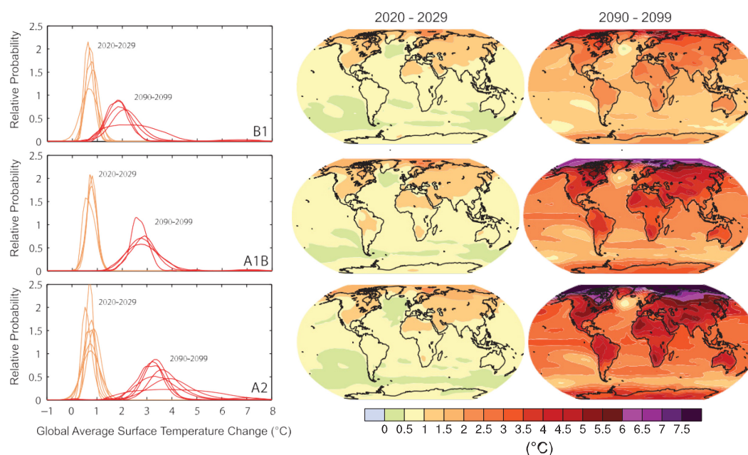
Figure 5.1. Projections of surface temperatures
