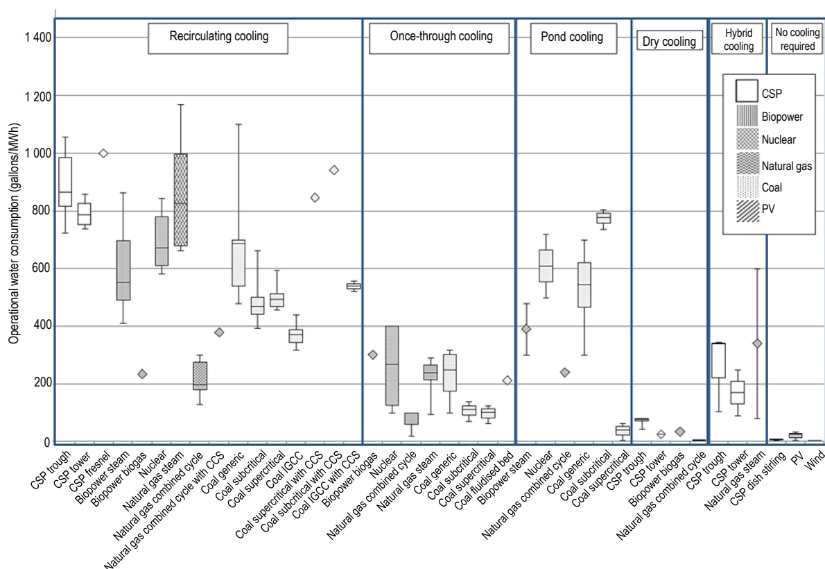
Figure 4.2. Operational water consumption factors for electricity generating technologies
