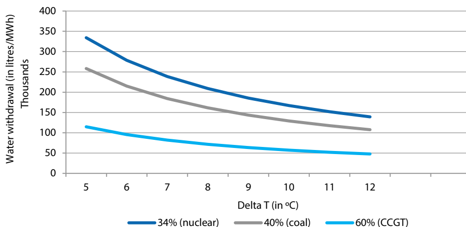
Figure 4.4. Water withdrawal rates required for once-through cooling of different thermo-electric plants, as a function of cooling water temperature rise
