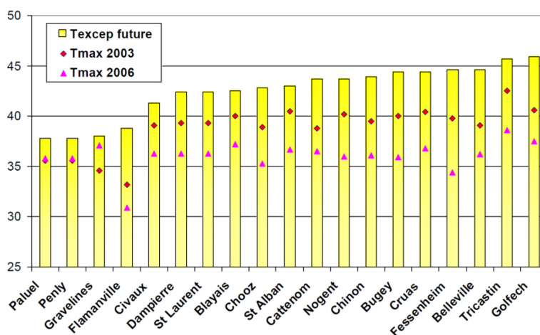
Figure 8.2. Evaluation of maximum air temperatures (°C) by the year 2030
