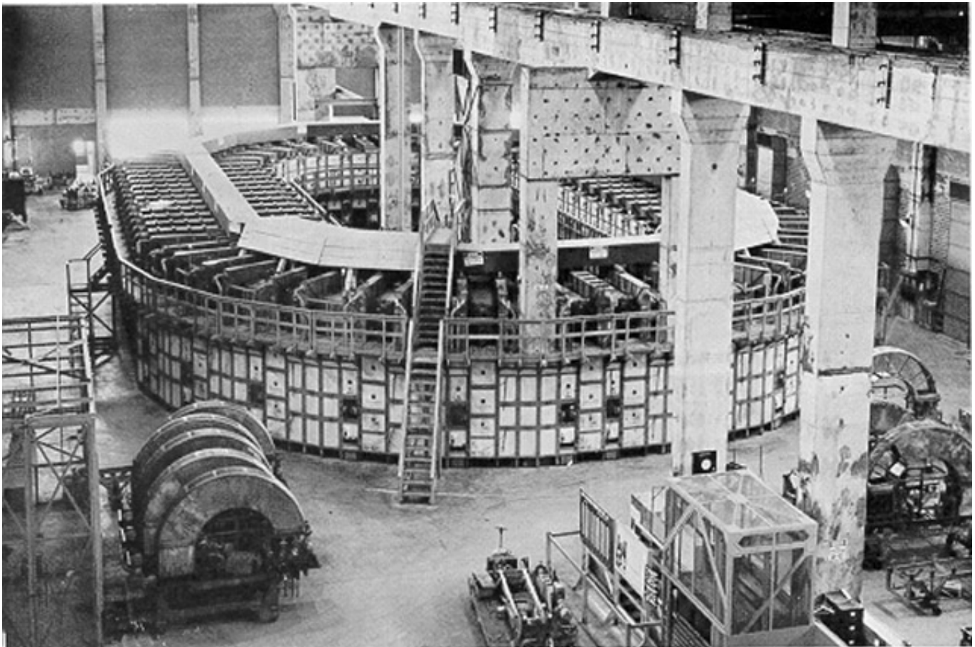
Figure 6: The electromagnetic separations plant built at Oak Ridge, Tennessee during the Manhattan Project. These devices, also referred to as calutrons, were used in enriching the uranium for the bomb that was dropped by the United States on Hiroshima. (photo taken from the website of the The Manhattan Project Heritage Preservation Association online at http://www.childrenofthemanhattanproject.org/OR/Photo-Pages/ORP-149.htm )
