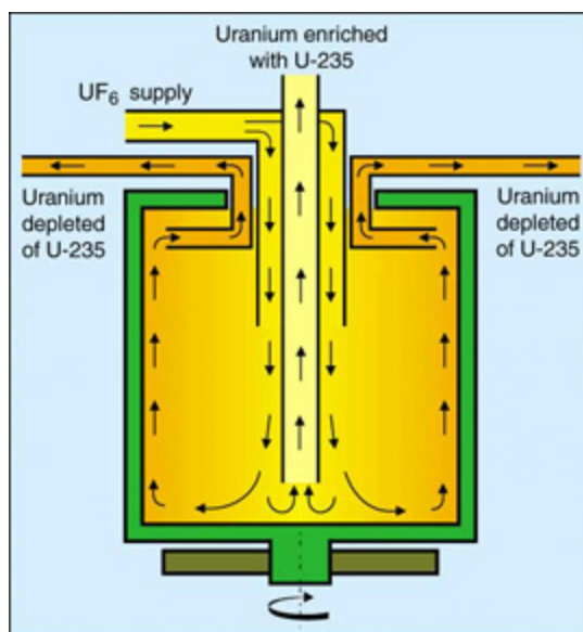
Figure 4: A schematic diagram of the cross section of a single gas centrifuge. The rotating cylinder forces the heavier U-238 atoms towards the outside of the centrifuge while leaving the lighter U-235 more towards the middle. A bottom to top current allows the enriched and depleted streams to be separated and sent via pipes to subsequent stages. (image taken from the website of the European Nuclear Society online at http://www.euronuclear.org/info/encyclopedia/images/gascentrifuge.jpg )
