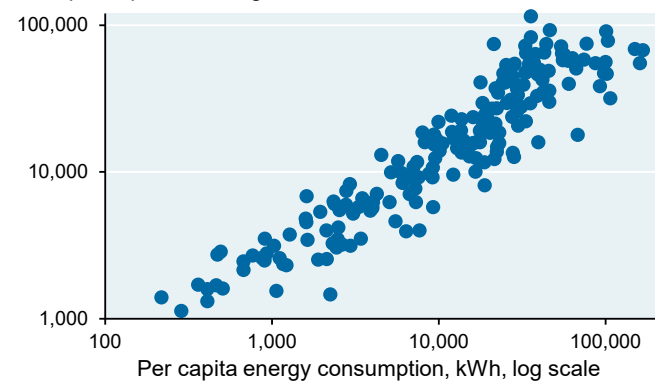
Per capita energy consumption and GDP by country
