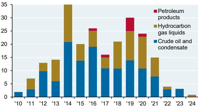
Annual US liquids pipeline project completions Number of projects
