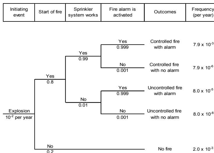
Figure 5-1 Example of an Event Tree Analysis
