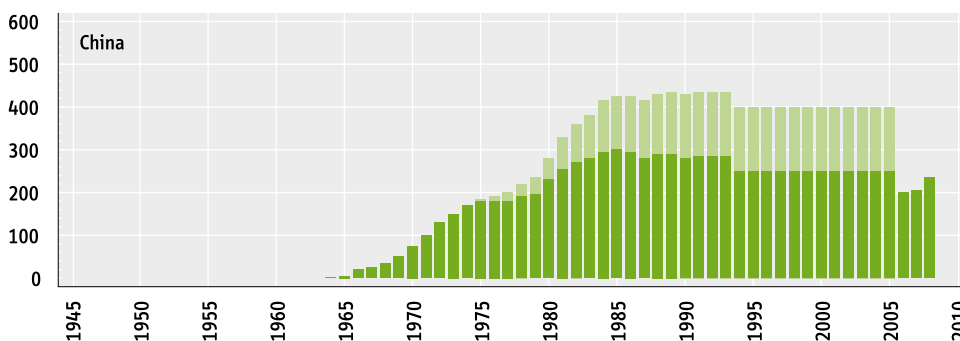
Figure 1.1. NRDC/FAS estimates of China’s total stockpile of nuclear weapons. In 2006, the NRDC/FAS experts revised their estimates for China after
