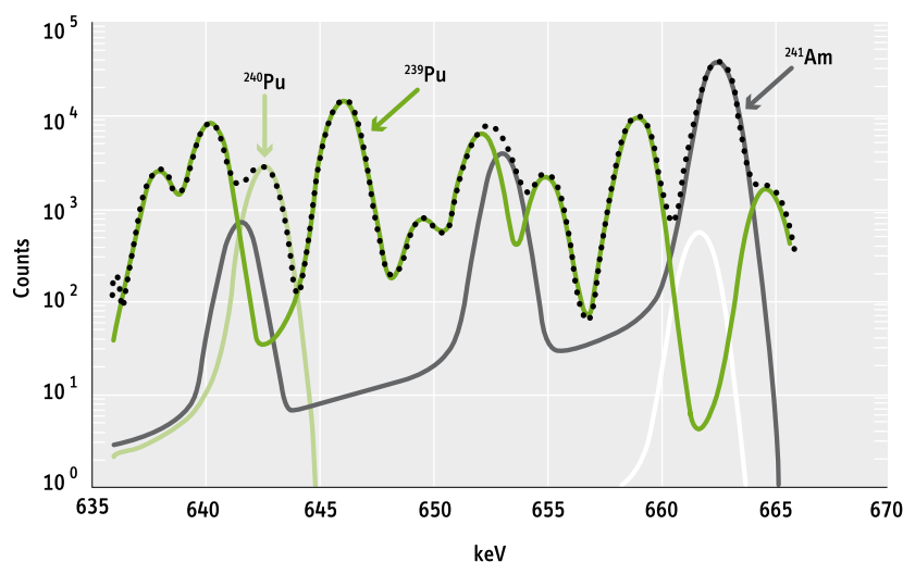
Figure 6.2. The 635 to 670-kilovolt region of the gamma-ray spectrum from plutonium contains emissions from both ^{239}\text{Pu} and ^{240}\text{Pu} . Precise measurements of the number of counts in each peak make it possible to establish the ratio ^{239}\text{Pu}/^{240}\text{Pu} and thereby the fact that the plutonium is weapon
