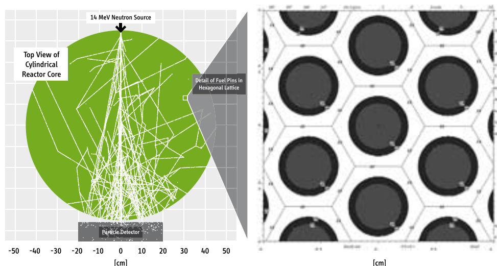
Figure 7.5. Notional submarine core and detector system. For simplicity, we assume that an entire reactor core would be placed within the detector system. The figure shows neutron tracks incident on the notional submarine reactor core. The neutron energy is assumed to be 14 MeV, and the detectors arranged around the core provide a trigger (top detector, not shown) and stop signal (bottom detector) for time-correlated measurements. Simulations demonstrate that approximately 3 % of the neutrons
