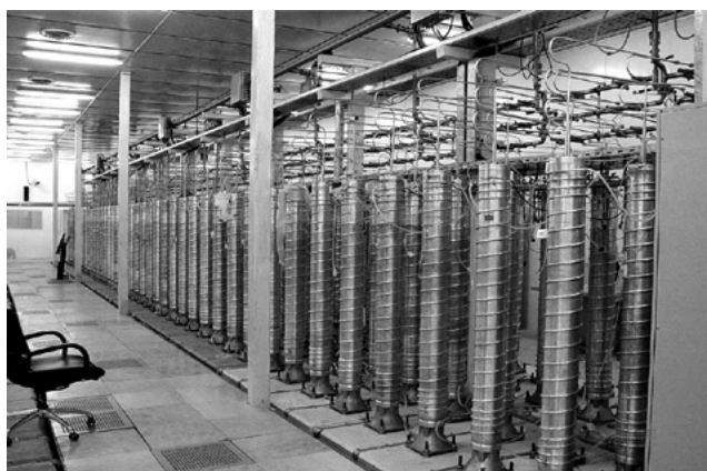
Figure 8.2. Iran's pilot plant with P1 centrifuges, 2005. 270
